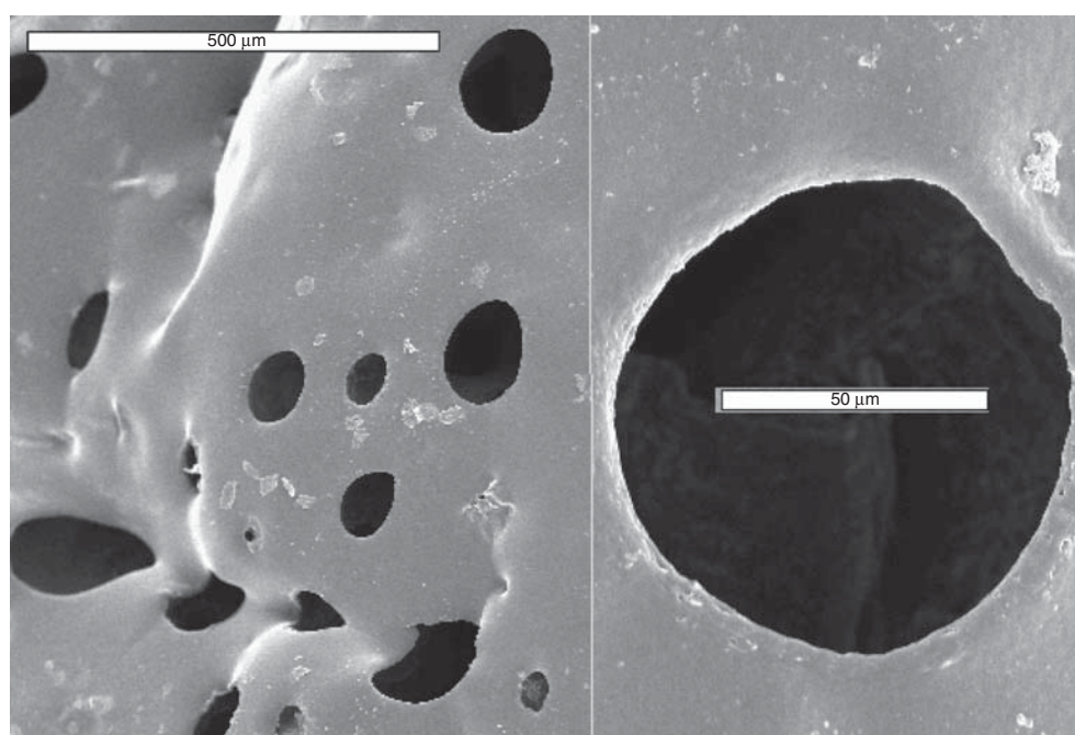
Figure 1. SEM micrograph of a superporous hydrogel hybrid.
